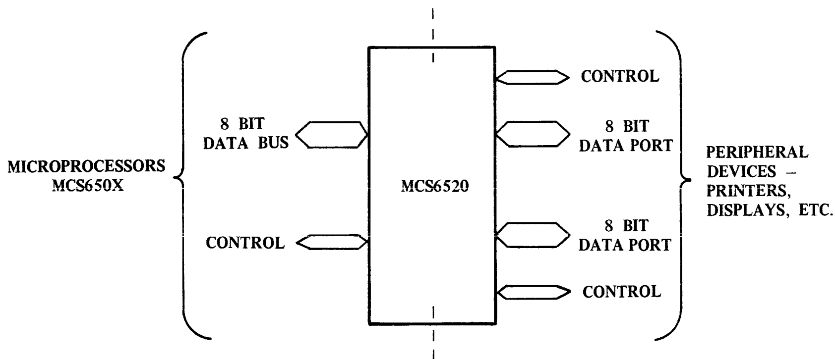
Basic MCS6520 Interface Diagram
